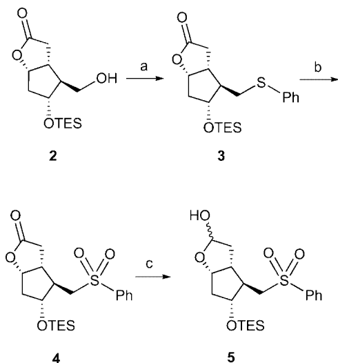
Scheme 2. The Synthesis of hemiacetal 5 . Reagents and conditions: a) DIAD, PPh 3 , PhSH, THF/CH 2 Cl 2 , 15–40 °C, 72%; b) (i) MMPP, H 2 O/CH 2 Cl 2 , 95%; (ii) crystallization, 79%; c) DIBALH, THF, –70 °C, 91.3%.
